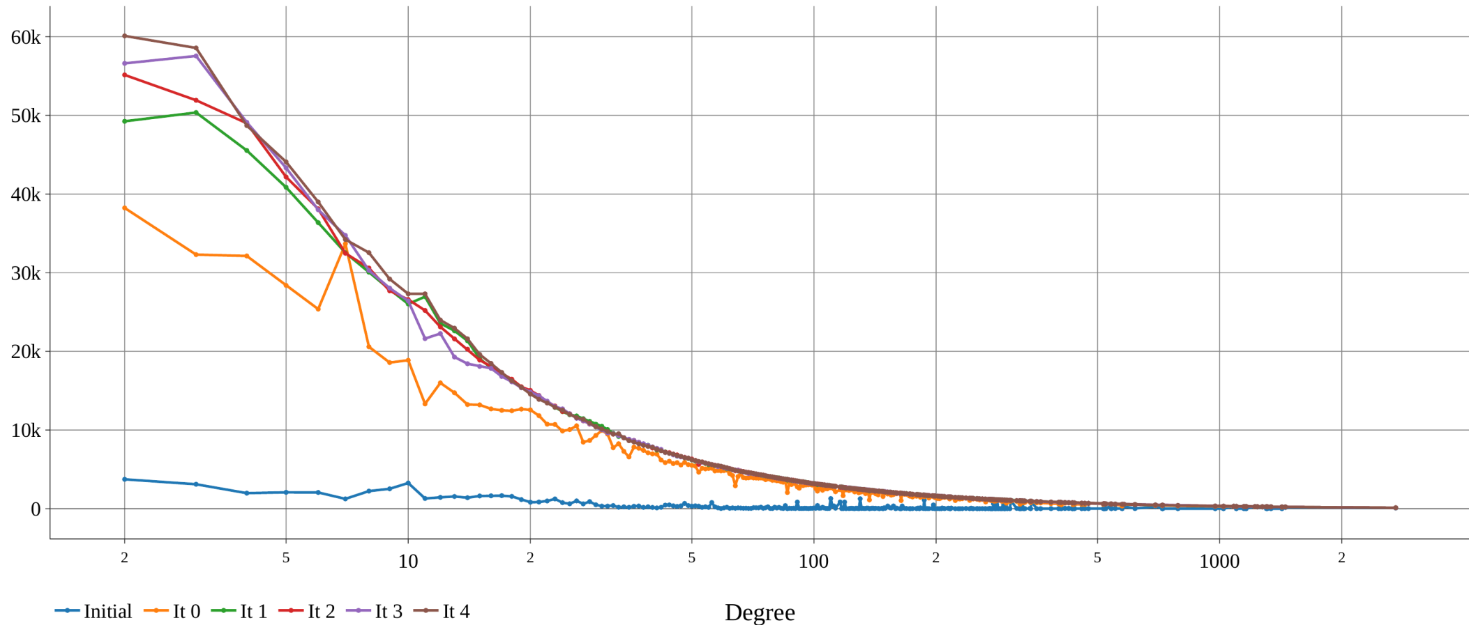
N2N AID, cnr-2000
