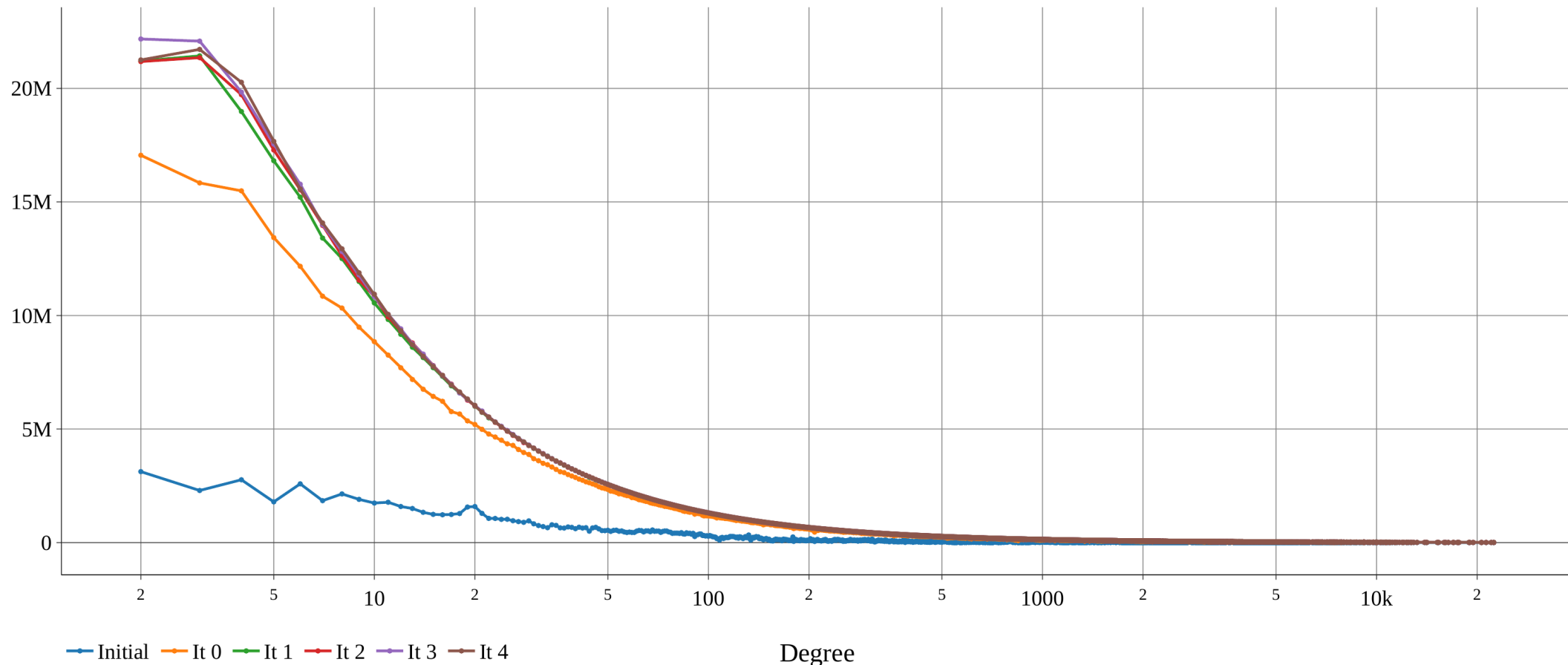
N2N AID, uk-union-2007
