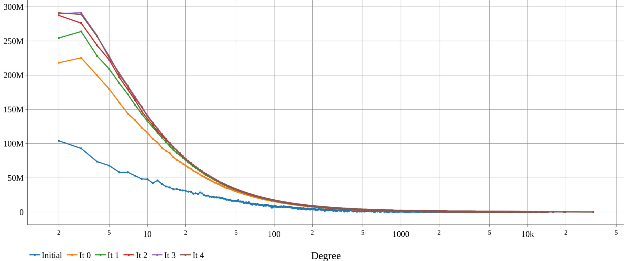
N2N AID, wdc14
