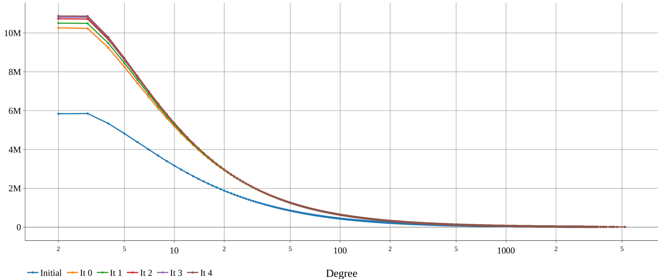
N2N AID, sym-friendster
