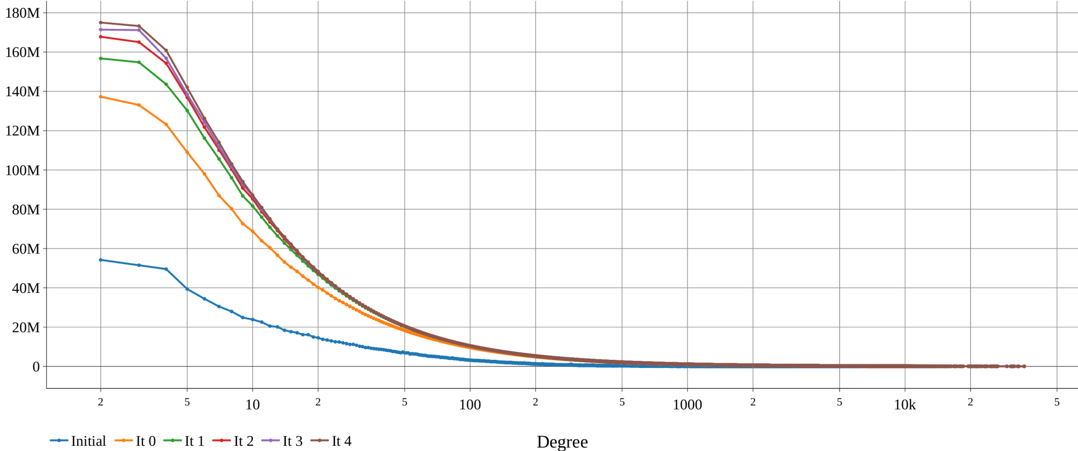
N2N AID, eu-2015
