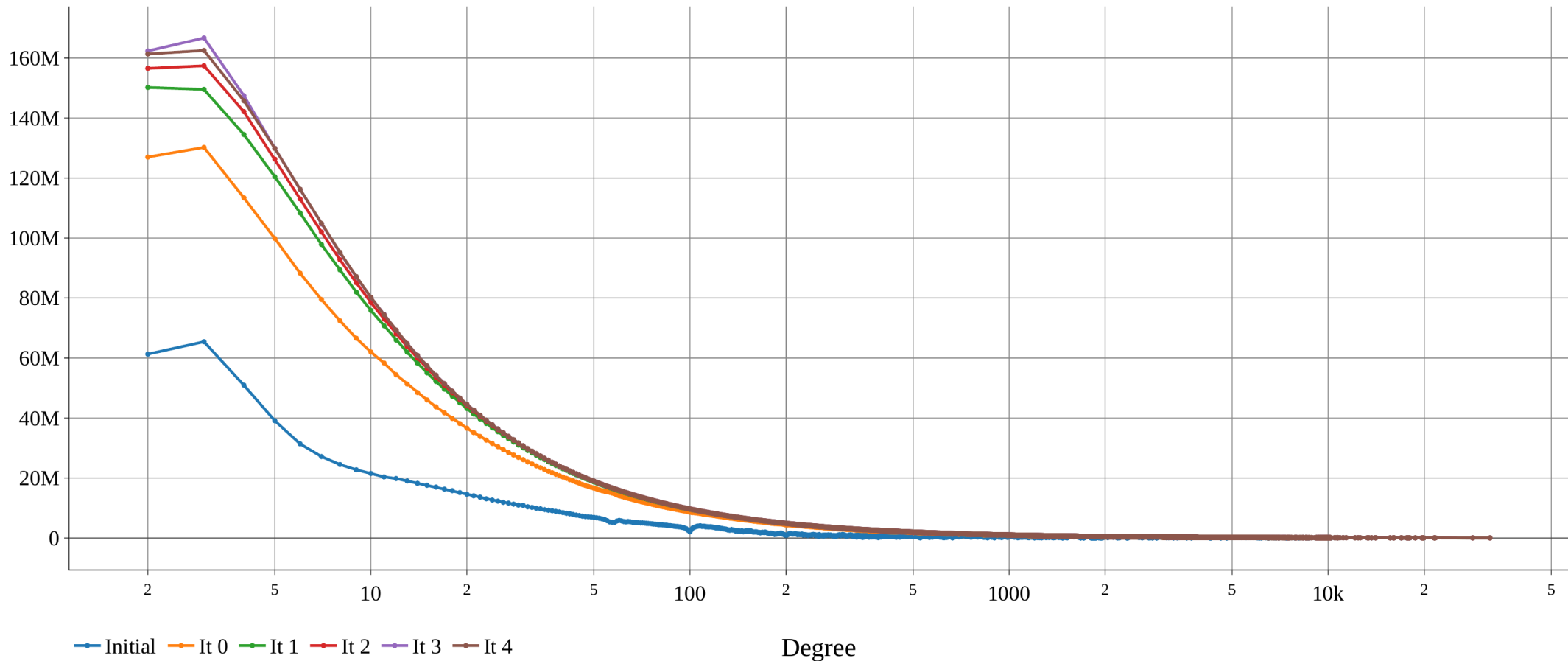
N2N AID, gsh-2015
